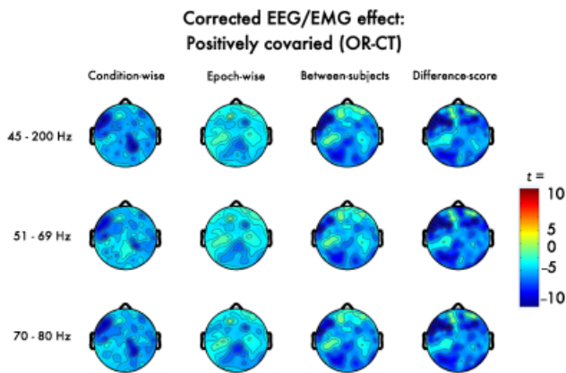
Figure 6. Thresholded ( p < .01 ) t -scores for the positively confounded eyes open, relaxed-closed, tense (OR-CT) contrast after EMG-residualization. At a qualitative level, only the epoch-wise method recovered the topography of the neurogenic effect (cf. Figure 2B).
