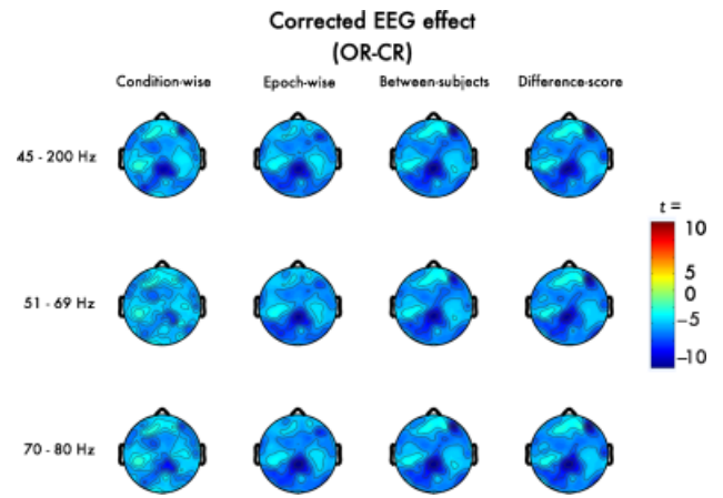
Figure 5. Thresholded ( p < .01 ) t -scores for eyes open-closed, relaxed (OR-CR) contrast after EMG-residualization.
