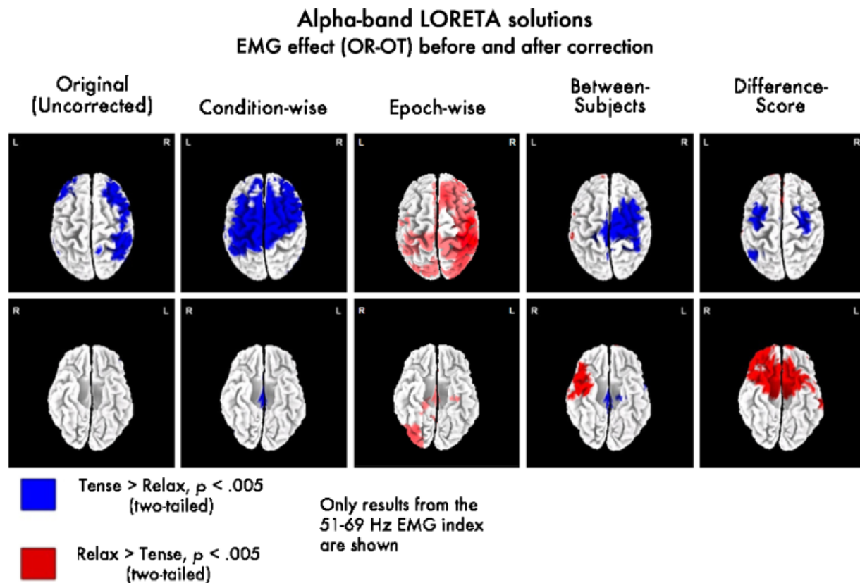
Figure 8. LORETA results. Thresholded ( p < .005 , uncorrected) eyes open relaxed-tense (OR-OT) contrast in the LORETA source-space rendered on the dorsal (top) and ventral (bottom) surfaces of a canonical brain. The left-most image depicts the uncorrected contrast (i.e., prior to EMG correction), followed by depictions (from left to right) of the effect after residualizing with the condition-wise, epoch-wise, between- and difference-score methods using the 51–69 Hz EMG band. Results (not shown) were similar for the other EMG bands.
