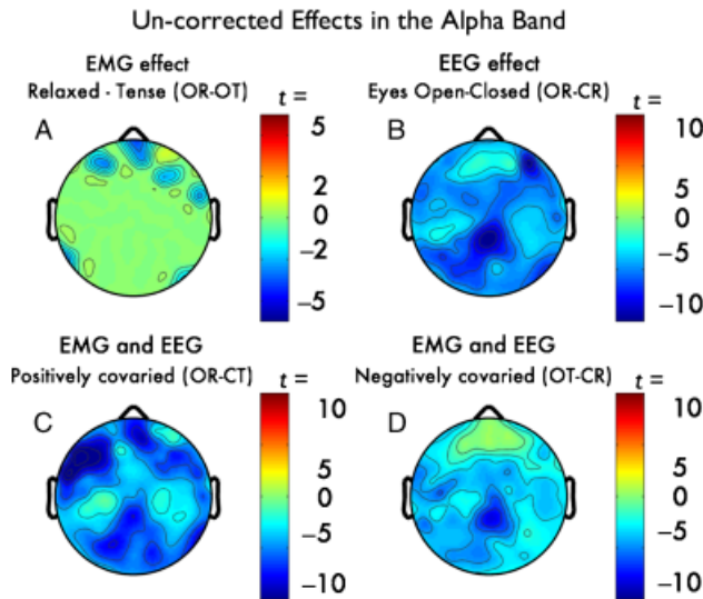
Figure 2. Thresholded ( p < .01 ) effects in the alpha-band (8–13 Hz) prior to EMG-correction. (A) The purely myogenic effect (OR-OT). Note the significant myogenic activation near the mastoids. (B) The alpha-blocking neurogenic effect (OR-CR). Note the roughly two-fold larger effect-size compared to the purely myogenic effect. (C) The effect of positively covaried EMG and alpha-blocking (OR-CT). Note the shift in the peak from the posterior midline to the left anterior region. (D) The effect of negatively covaried EMG and alpha-blocking (OT-CR). Abbreviations are described in the Method section.
