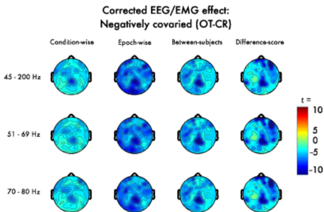
Figure 7. Thresholded ( p < .01 ) t -scores for the negatively confounded eyes open, tense-closed, relaxed (OT-CR) contrast after EMG-residualization. Note the poor sensitivity of the condition-wise technique.
