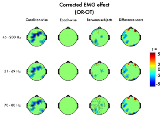
Figure 4. Thresholded ( p < .01 ) t -scores for the eyes open relaxed-tense (OR-OT) contrast after EMG-residualization. Note the relatively poor performance of the condition-wise method.
