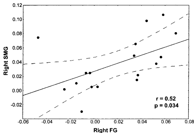
FIG. 5. Pearson's correlation between differential activity (liked-minus-disliked) within the right supramarginal gyrus (y axis) and the right FG (x axis). FG cluster defined by the meta-cluster common to prior fMRI studies. Units scaled to \text{A/m}^2 . Dotted lines: \pm 95\% confidence intervals.
