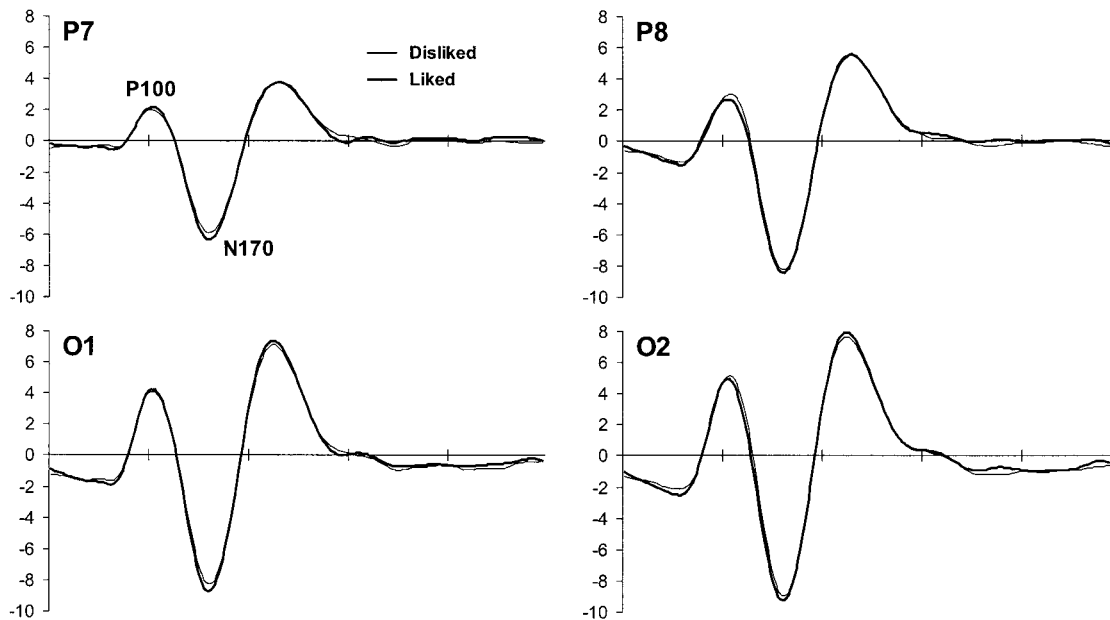
FIG. 3. Grand mean ERP ( n = 17 ) waveforms evoked by liked (thick lines) and disliked (thin lines) faces at P7, P8, O1, and O2. Horizontal: time in milliseconds (from 0 to 500 ms poststimulus); vertical: amplitude in microvolts. At P7, the P100 and N170 components are shown.
