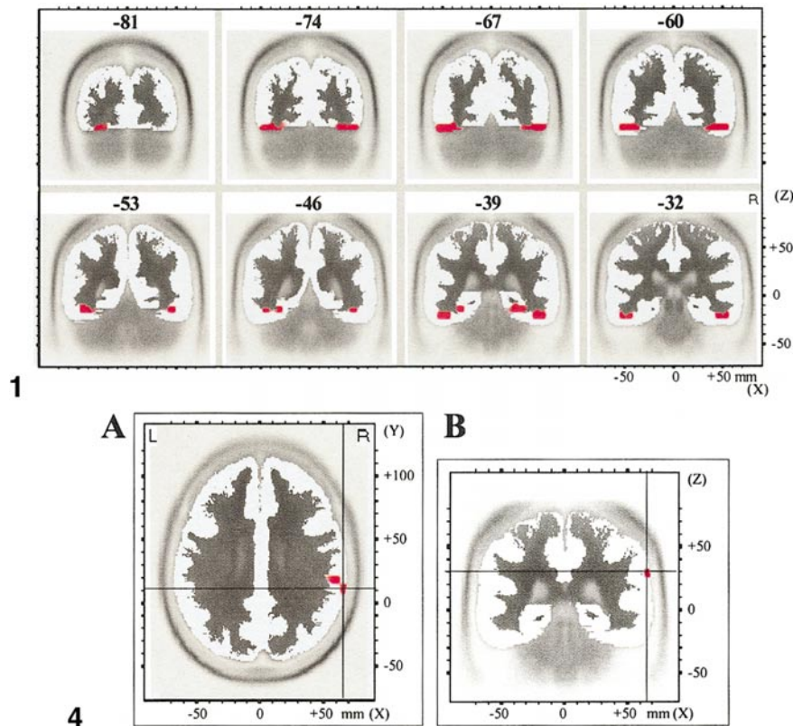
FIG. 1. Coronal slices (from y = -81 , most posterior, to y = -32 , most anterior) showing the location and spatial extent of (and not the activation level in) the FG cluster (red) as defined by the Structure-Probability Maps (Lancaster et al. , 1997). Origin at anterior commissure; (X) = left(–) to right(+); (Y) = posterior(–) to anterior(+); (Z) = inferior(–) to superior(+). In Figs. 1 and 2, the right hemisphere is shown on the right-hand side.
