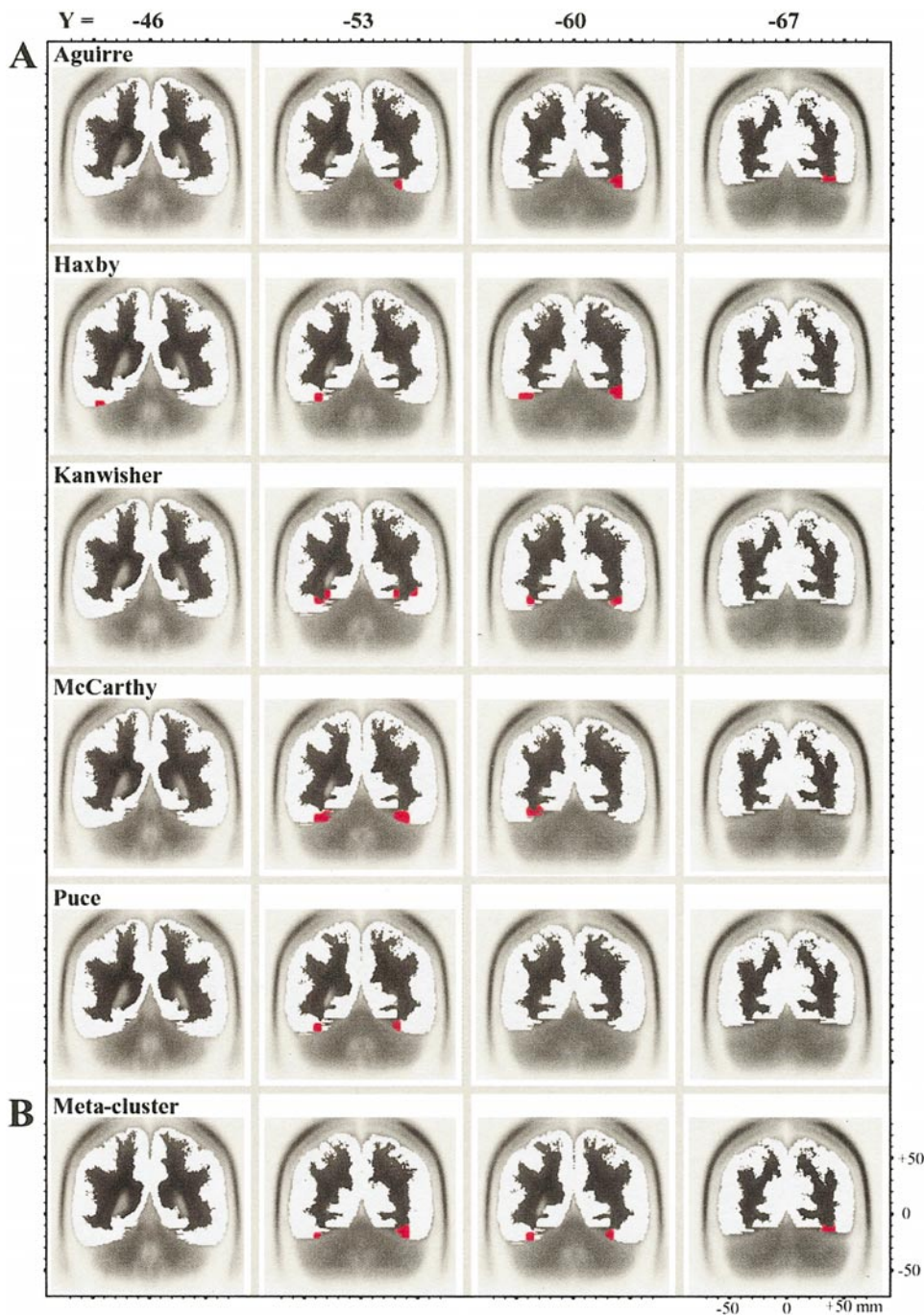
FIG. 2. Coronal slices (from y = -67 , most posterior, to y = -46 , most anterior) showing the location and spatial extent of (and not the activation level in) the fusiform gyrus in LORETA space. All voxels needed to approximate the face-sensitive fMRI coordinates through interpolation are shown. (A) ROIs defined by the coordinates of prior fMRI studies (Puce et al. , 1996; Kanwisher et al. , 1997; McCarthy et al. , 1997; Aguirre et al. , 1999; Haxby et al. , 1999); (B) ROIs defined by the meta-cluster common to prior fMRI studies.
