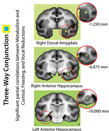
Fig. 3. Shared neural substrates: Amygdalar and hippocampal metabolism predicts all three dimensions of the AT phenotype. Figure depicts the three-way minimum conjunction (logical AND) of the significant partial correlations shown in Fig. 2. Regions shown in cyan/gold predicted the unique variance in all three dimensions of the AT phenotype. Circular insets show magnified views. For other conventions, see Fig. 2.
