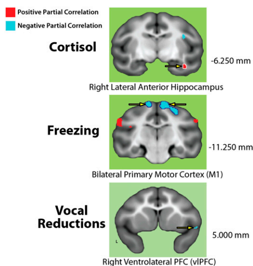
Fig. 4. Selective substrates: Regions where one AT dimension predicted significant variance in brain metabolism (partial correlation: FDR q < 0.05 ) and explained more variance than the other two dimensions (difference in correlations: FDR q < 0.05 ), identified using a two-way conjunction (logical AND). Conventions are described in Fig. 2.
