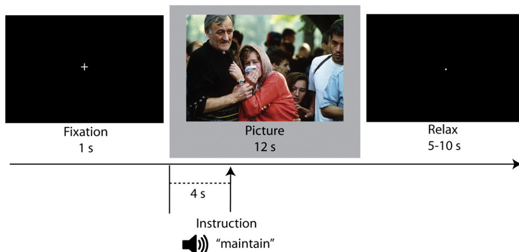
Fig. 1. Trial structure for the reappraisal task. One instruction (increase, maintain or decrease) was delivered 4 s after picture onset on each trial. This figure represents a “maintain” trial. Photo of mourning family by Mikhail Evstafiev retrieved from http://commons.wikimedia.org/wiki/File:Evstafiev-bosnia-sarajevo-funeral-reaction.jpg on August 18, 2008. It is licensed under the Creative Commons Attribution ShareAlike 2.5 License, which allows reproduction (see license at http://creativecommons.org/licenses/by-sa/2.5 ).
