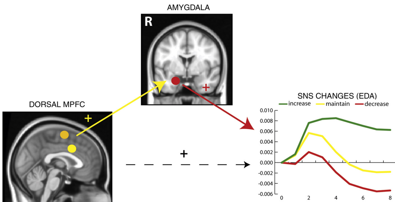
Fig. 4. This simple framework depicts the information processing taking place during reappraisal and its associated medial prefrontal neural correlates in the present study, as supported by mediation analyses. We propose that reappraisal-related activation in two regions of dorsal medial prefrontal cortex (MPFC; shown with yellow circles: dorsal medial frontal gyrus, top circle, and dorsal cingulate gyrus, bottom circle) (increase, decrease > maintain) carries out information processing associated with the cognitive demand involved in reappraisal. This activation produces monotonic change in the right amygdala (linear contrast score: increase > maintain > decrease; shown with red circle), which monitors the need for energy mobilization due to changes in motivational state. Amygdala changes then facilitate sympathetic nervous system (SNS) output, signifying changes in emotional arousal (also using linear contrast score) that accord with the regulatory goal. The black arrow connecting dorsal MPFC with SNS activation is broken so as to communicate the fact that this direct association is reduced or eliminated when taking the amygdala into account.
