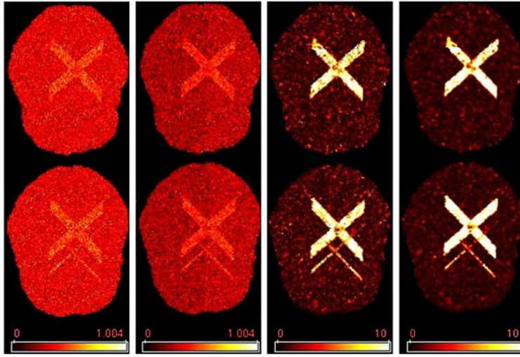
FIG. 7. Comparison of color maps for simulated data set. From left to right: FA; Smooth-FA; -\log(p) by \mathbb{K} ; -\log(\tilde{p}) by \mathbb{K} . SNR = 10.
